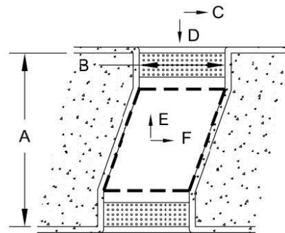
CT TYPE 4 STAGGERED ISLAND
