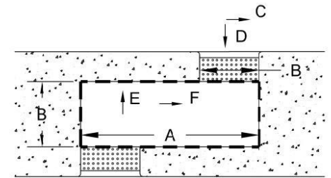
CT TYP 5 STAGGERED "L" ISLAND
